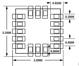
Figure 111. Recommended Printed Wiring Board Land Pattern (Dimensions Shown in Millimeters)
