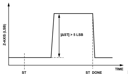
Figure 112. Self Test Waveform
